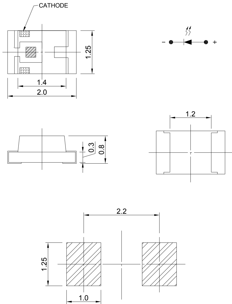
Recommended soldering Pad
